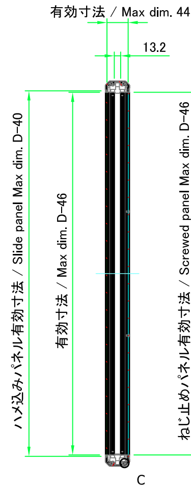
B-B (1:8)
